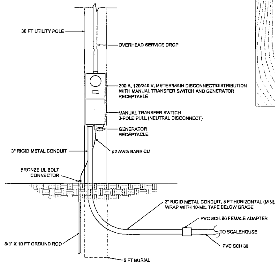
UTILITY METER/MAIN DISCONNECT WITH MANUAL TRANSFER SWITCH (18) NOT TO SCALE 14/14
