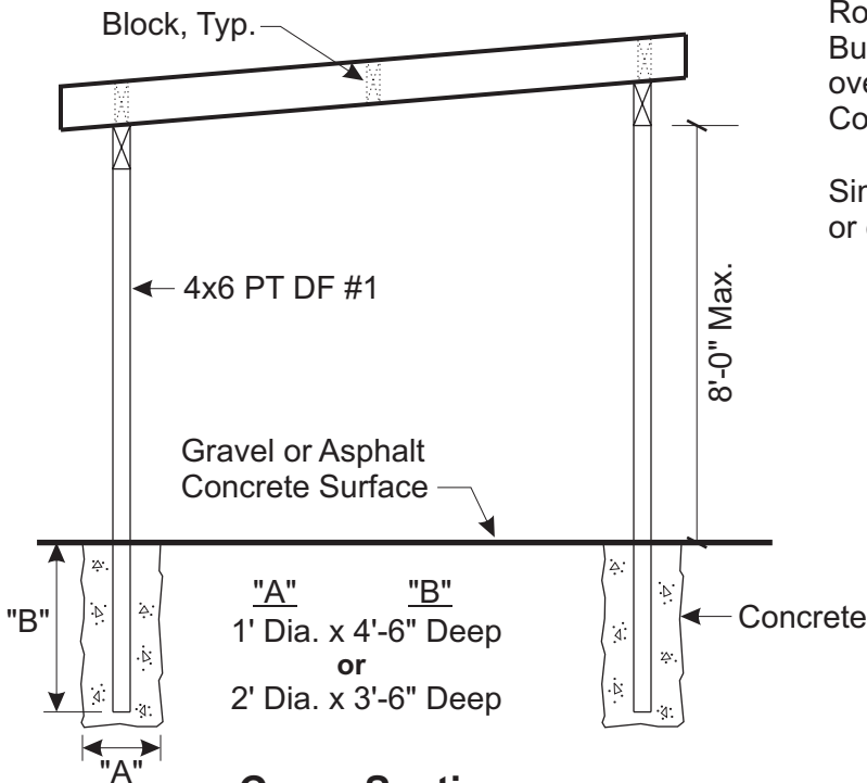
Cross Section
