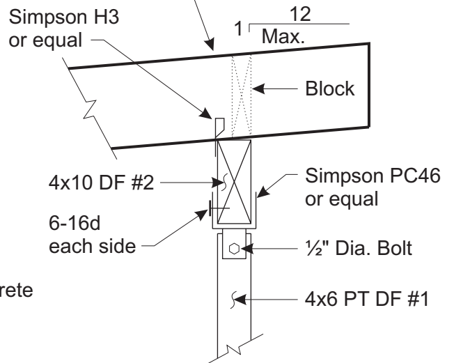
Roof to Post Detail
