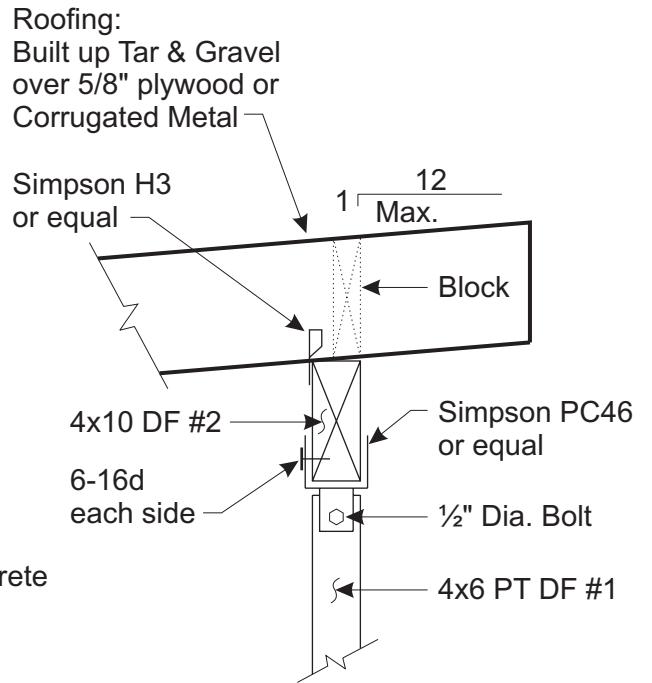
Roof to Post Detail
