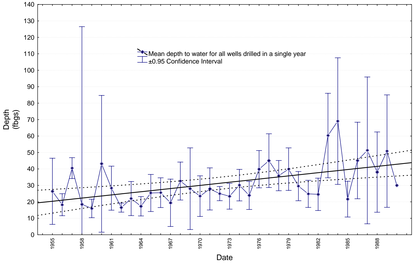
Figure 3: Depth to Water In New Wells Over Time Joy Road Study Area
